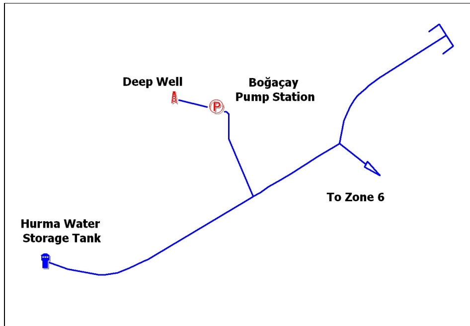
Figure 6.6 Simplified Schematic Drawing of Konyaalti Water Transmission System and Zone 6 Entrance
