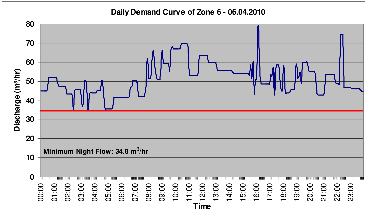
Figure 6.35 Daily Demand Curve of Zone 6 on 06.04.2010
