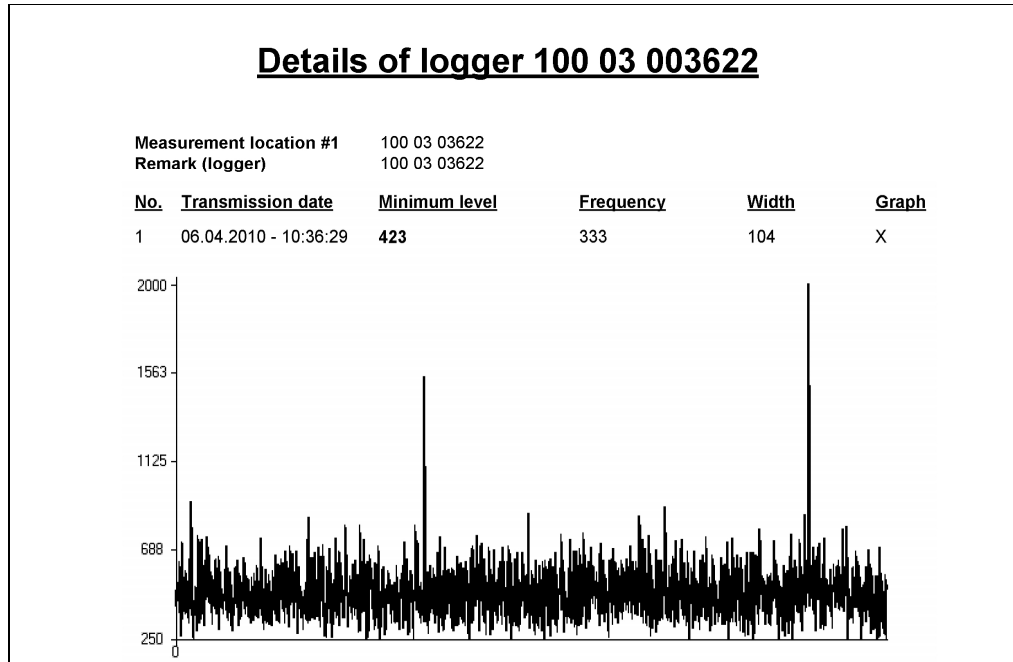
Figure 6.23 Details of Logger with Serial Number 3622 Placed On Valve #27104
