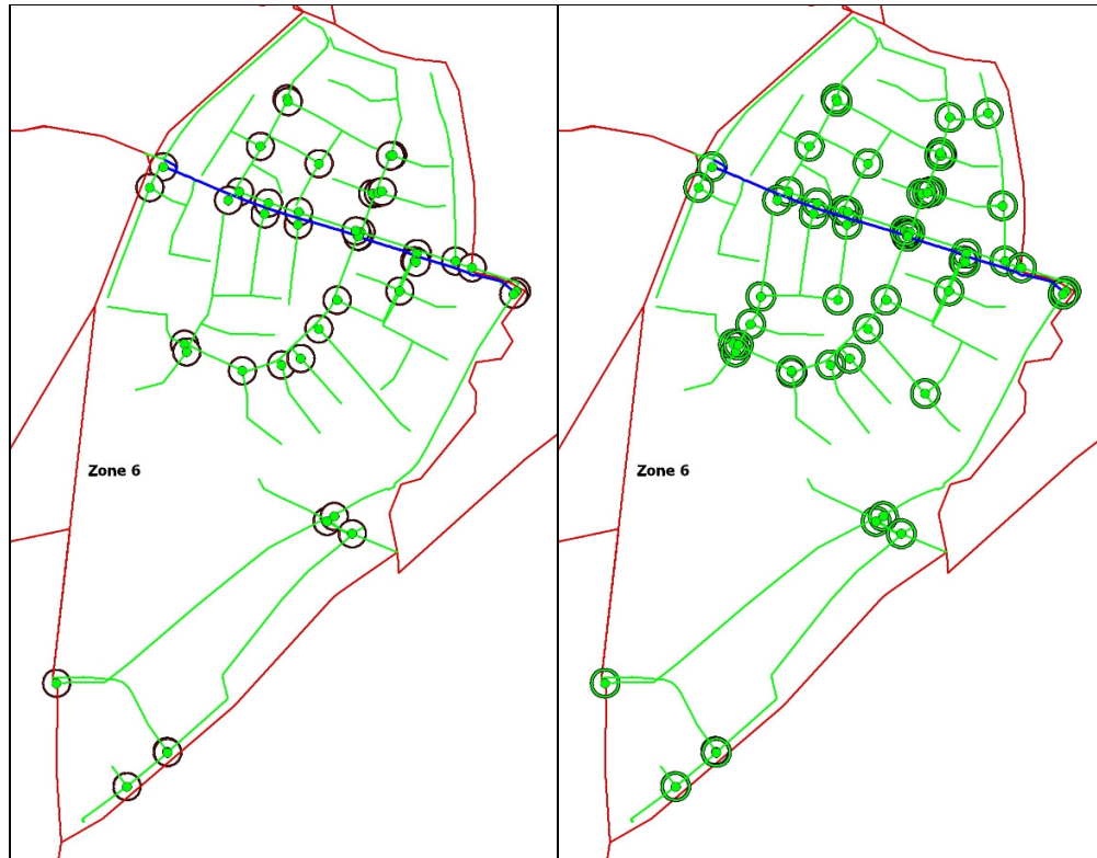
Figure 6.9 Valves and Their Effective Areas Before and After Constructions
