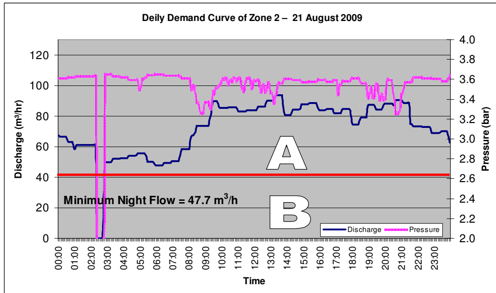
Figure 6.45 Sample Daily Demand Curve of Zone 2 Showing Minimum Night Flow on 21 August 2009
