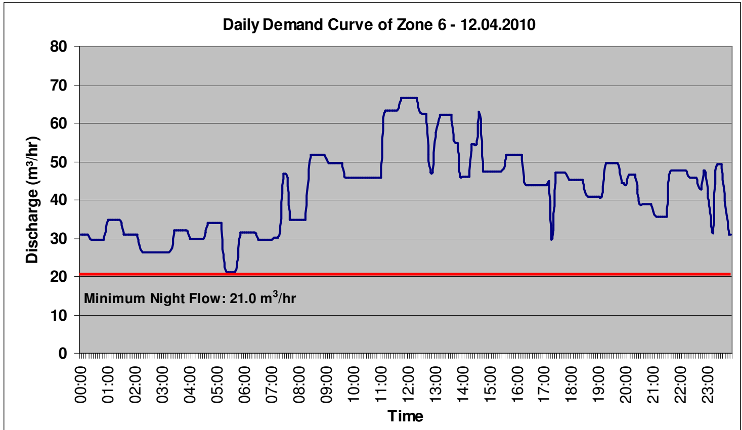
Figure 6.38 Daily Demand Curve of Zone 6 on 12.04.2010
