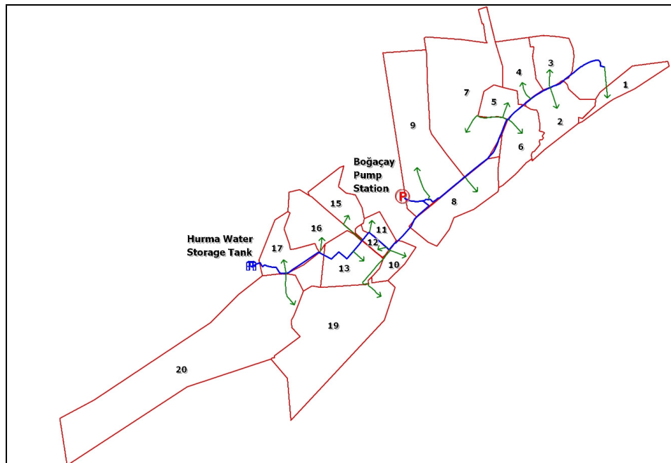
Figure 6.7 Distribution Main of Konyaalti and Branching Pipes of 18 DMAs
